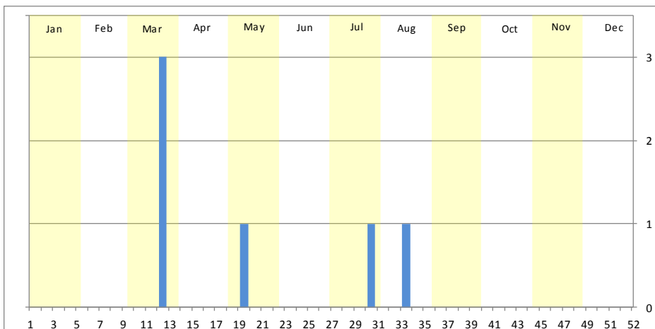
Figure 2: Little Ringed Plover records at Folkestone and Hythe by week
