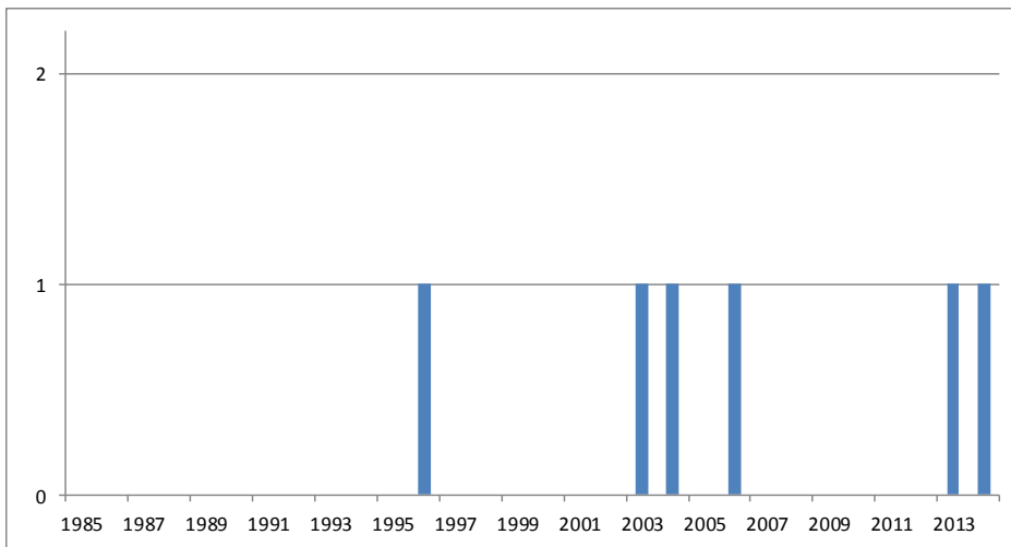
Figure 1: Little Ringed Plover records since 1985 at Folkestone and Hythe
